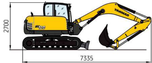
Fig. 2: Transport position
